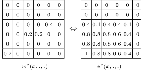
FIG. 4.1. On the left: example of values w^*(x, \dots) . On the right: corresponding values \phi^*(x, \dots) .
