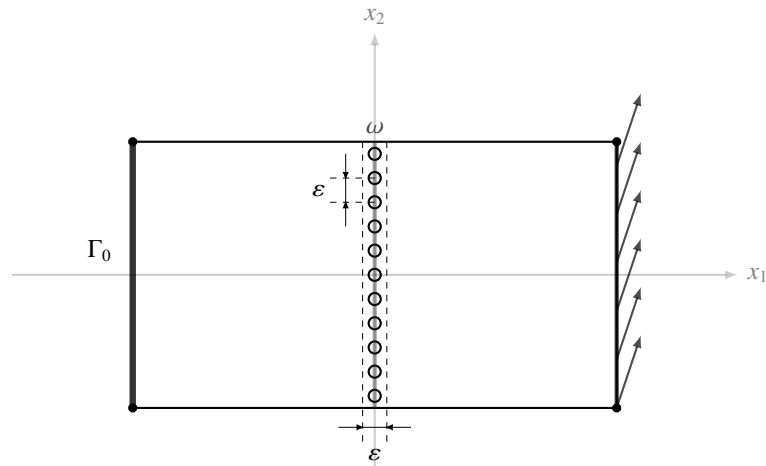
Fig. 8. Test Problem
