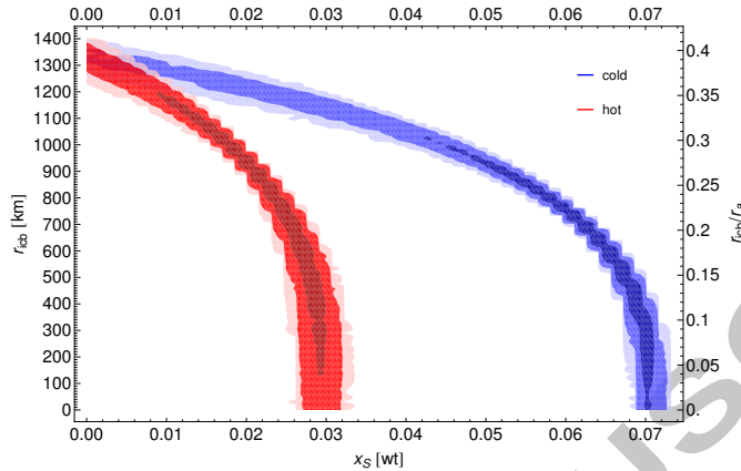
Figure 7: Inner core size as function of sulfur weight fraction for the hot and cold mantle temperature. Contours delimit domains corresponding to 0.997, 0.954, 0.682 probability of occurrence.
