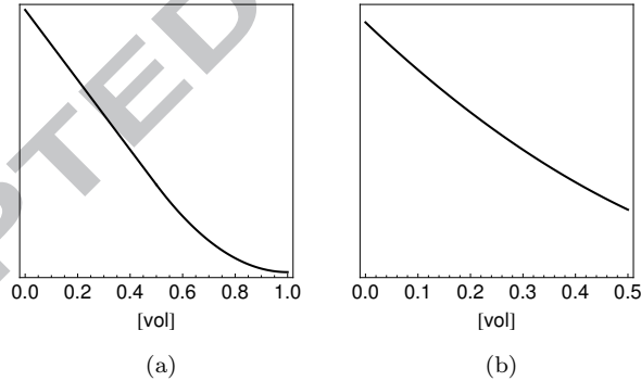
Figure 4: Marginal prior probability density functions for olivine, orthopyroxene, and garnet (a) and Ca-pyroxene (b).
