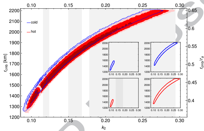
Figure 8: Core size as function of k_2 for the hot and cold mantle temperature for models that satisfy the MOI . Contours delimit domains corresponding to 0.997, 0.954, 0.682 probability of occurrence. The gray shaded areas represent the k_2 values of Marty et al. (2009) , Konopliv et al. (2011) , and Smith et al. (2009) (from left to right). The insets correspond to the individual 0.997 contours of the models with an inner core and without an inner core for cold and hot mantle models.
