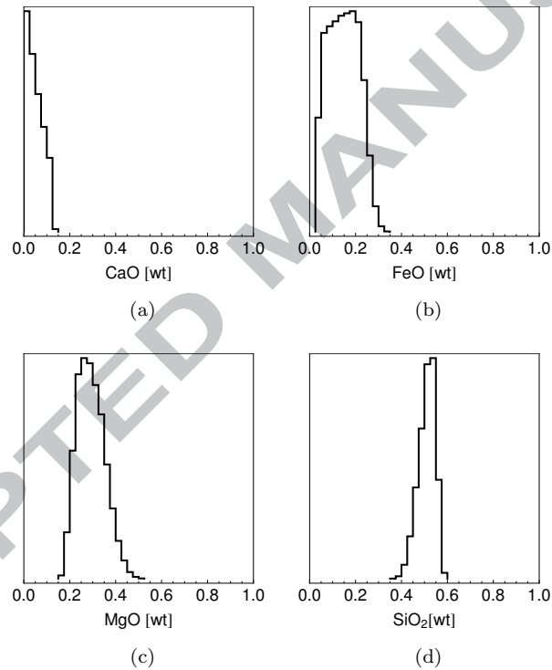
Figure 5: Probability density functions of mass fractions of CaO (a), FeO (b), MgO (c), and SiO 2 (d).
