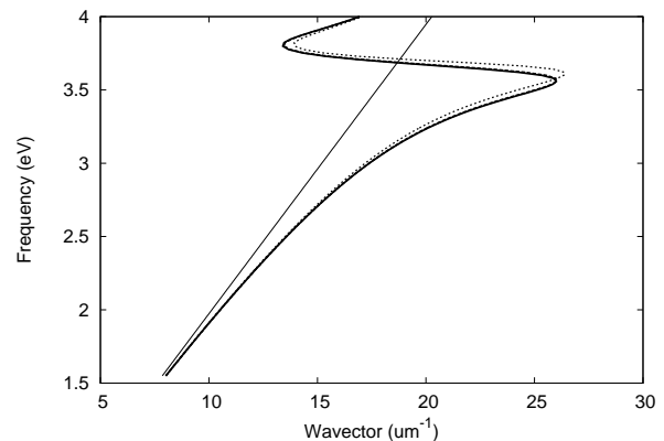
FIG. 4. Dispersion relation ( \omega as a function of k_x ) for a surface plasmon at the interface between silver and air. The local description (thick solid curve) can almost not be distinguished from the nonlocal description (thick dashed curve, almost identical with the thick solid curve). In order to illustrate the effect of nonlocality, we show here (dotted line) the impact of an exaggerated nonlocality ( \beta multiplied by ten). The thin solid curve is \omega = k_x c .
