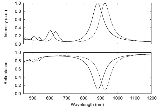
FIG. 11. Bottom : Reflection spectrum according to local (RCWA, dashed line) and nonlocal (COMSOL, solid line) simulations. Top : Model (57) for the field intensity under the strips for the local (dashed line) and nonlocal (solid line) theory. The agreement between the simulations and the model are in excellent agreement for the local as well as for the non-local theory.
