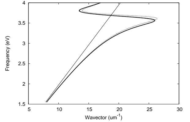
FIG. 4. Dispersion relation ( \omega as a function of k_x ) for a surface plasmon at the interface between silver and air. The local description (thick solid curve) can almost not be distinguished from the nonlocal description (thick dashed curve, almost identical with the thick solid curve). In order to illustrate the effect of nonlocality, we show here (dotted line) the impact of an exaggerated nonlocality ( \beta multiplied by ten). The thin solid curve is \omega = k_x c .
