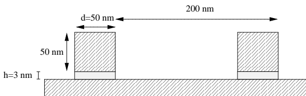
FIG. 10. Strips (rods with a 50 nm by 50 nm section) are separated from the metallic film by a 3 nm thick dielectric with an optical index of 1.58. The structure considered here is periodic, with a 200 nm period.
