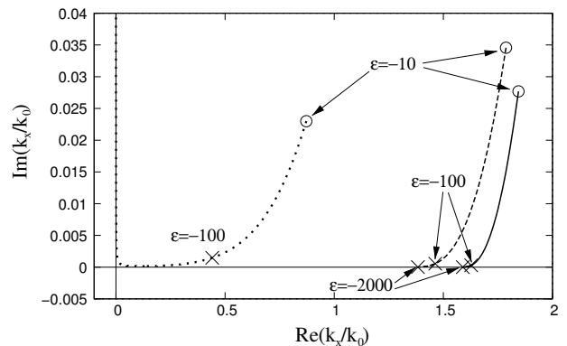
FIG. 6. Trajectory in the complex plane of the quantity \frac{k_x}{k_0} for three different waveguided modes (solid line: first even mode; dashed line: first odd mode ; dotted line: second even mode) when the permittivity of the metal goes from \epsilon = -10 + i (circles) to \epsilon = -2000 + i , for a thickness of the waveguide of 500 nm and a dielectric with an 1.58 optical index. The intermediate value of -100 + i is indicated on the curves.
