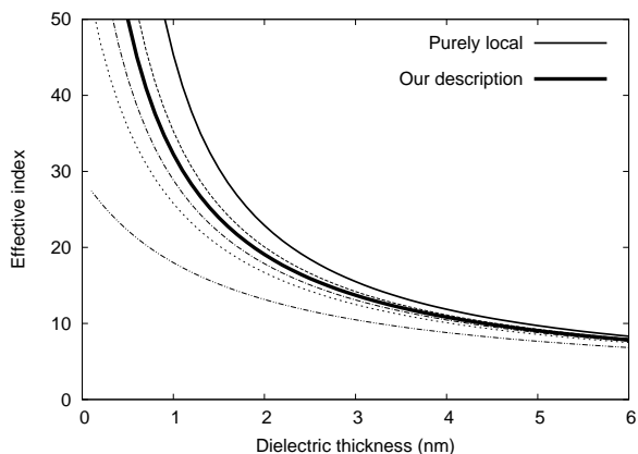
FIG. 8. Effective index of the guided mode at 600 nm, as a function of the dielectric width, h . The dispersion relations are shown for different descriptions (see table I): the completely local case (thin black curve, top), P_z(0) = 0 (description 1, dash-dotted line) and E_z continuous (description 2, dashed line) with no identified contribution of the bound electrons, and descriptions separating the contributions of bound and free electrons, with P_z = 0 (description 3, dash-double dotted line), a continuous E_z (description 4, thin dash line) and finally our description (description 5, thick solid curve), that is preferred in this work.
