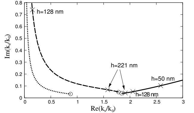
FIG. 7. Trajectory in the complex plane of the quantity \frac{k_x}{k_0} for three different waveguided modes (solid line: first even mode; dashed line: first odd mode; dotted line: second even mode) when the width of the metal goes from 380 nm (circles) to 10 nm. The permittivity of the metal is taken equal to the permittivity of gold at 608 nm, \epsilon \simeq -10.01 + 1.44i . Intermediate thickness of 221 nm (when the real part of the index of the odd mode becomes smaller than 1.58, so that the coupled plasmon picture becomes less relevant), 128 nm (when the odd mode can be considered non-propagative, and the coupled plasmon picture is not relevant any more) and 50 nm are indicated on the curves.
