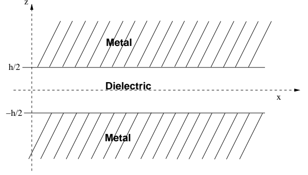
FIG. 5. Metallic waveguide of width h .
