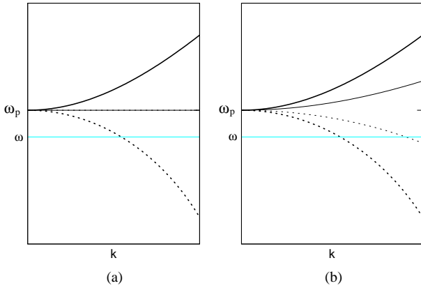
FIG. 2. Dispersion relation for transverse waves (thick lines) and bulk plasmons (thin lines) when (a) the nonlocality is absent ( \beta = 0 ) and (b) the nonlocality is important. The dashed lines show the imaginary parts of the propagation constants for the transverse and longitudinal waves, below the plasma frequency \omega_p . When nonlocality is present, for a given \omega two waves must be taken into account.(color online)
