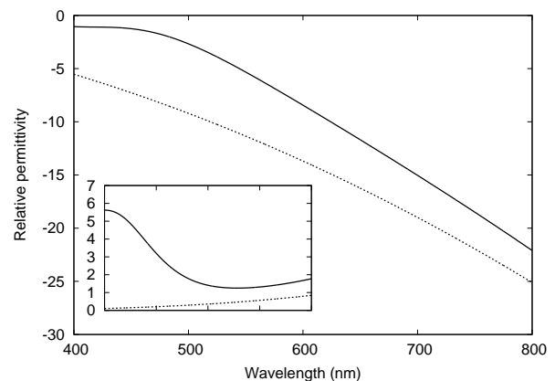
FIG. 1. Real part of the relative permittivity of gold in the visible (solid line) and Drude permittivity according to 39 (dotted line). The difference is the contribution of bound electrons. Inset : imaginary part of the relative permittivity, same x scale, same lines.
