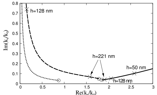
FIG. 7. Trajectory in the complex plane of the quantity \frac{k_x}{k_0} for three different waveguided modes (solid line: first even mode; dashed line: first odd mode ; dotted line: second even mode) when the width of the metal goes from 380 nm (circles) to 10 nm. The permittivity of the metal is taken equal to the permittivity of gold at 608 nm, \epsilon \simeq -10.01 + 1.44i . Intermediate thickness of 221 nm (when the real part of the index of the odd mode becomes smaller than 1.58, so that the coupled plasmon picture becomes less relevant), 128 nm (when the odd mode can be considered non-propagative, and the coupled plasmon picture is not relevant any more) and 50 nm are indicated on the curves. .
