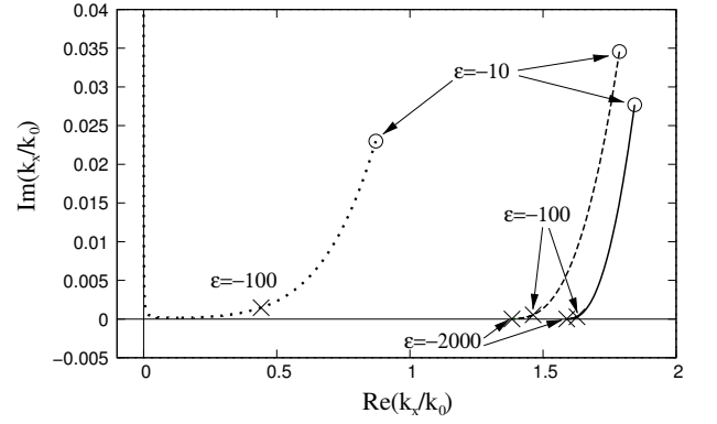
FIG. 6. Trajectory in the complex plane of the quantity \frac{k_x}{k_0} for three different waveguided modes (solid line: first even mode; dashed line: first odd mode; dotted line: second even mode) when the permittivity of the metal goes from \epsilon = -10 + i (circles) to \epsilon = -2000 + i , for a thickness of the waveguide of 500 nm and a dielectric with an 1.58 optical index. The intermediate value of -100 + i is indicated on the curves.
