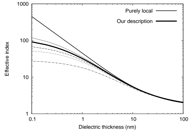
FIG. 9. Same as figure 8 except for the log scale.
