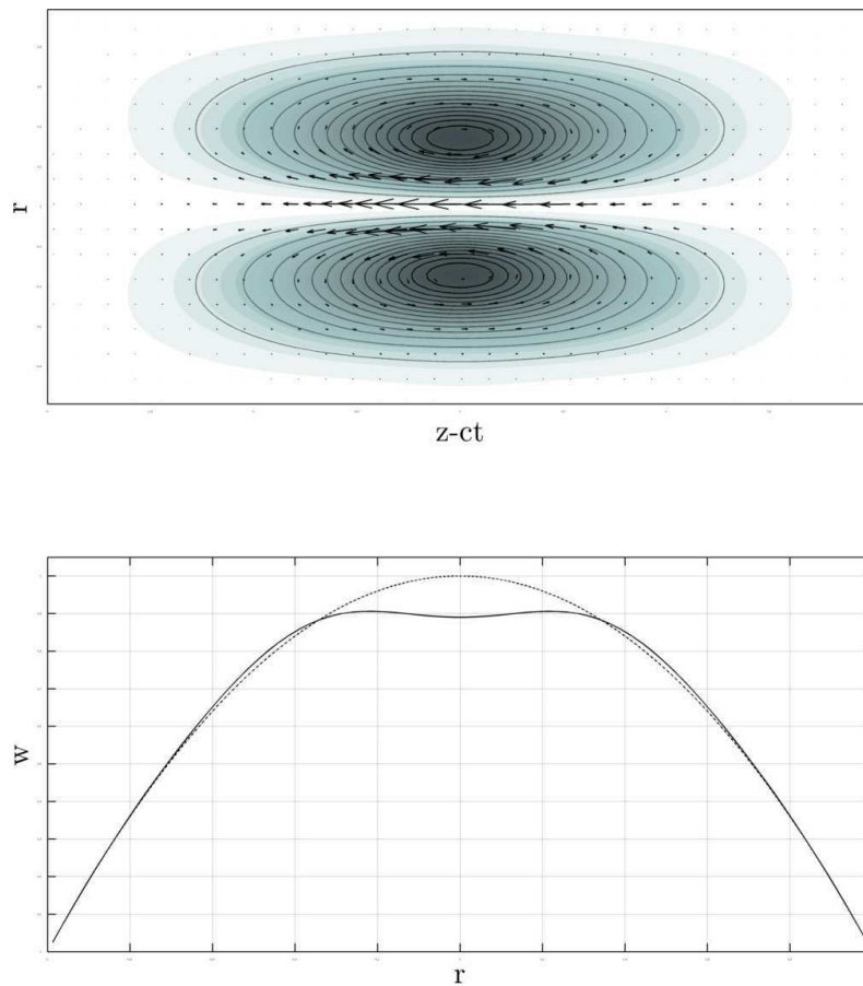
FIGURE 2. Centre vortexon: (top) streamlines of the three-component KdV solution and (bottom) velocity profiles of the perturbed (solid) and laminar (dash) flows ( c = 0.62 , q = 0 ).
