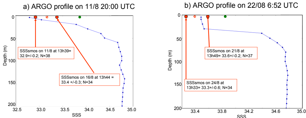
Fig. 4. Two successive ARGO profiles taken by float 4900325 (blue curve) on (a) 11 August 20:00 UTC (latitude = 12.4° N; longitude = 117.6° W) and (b) 22 August 6:52 UTC (latitude: 12.2° N; longitude: 117.8° W). Mean SMOS SSS collocated with these profiles in a radii of 5 day and 50 km are indicated by red dashed point. In each case, two SMOS passes have participated to these collocations: mean SMOS SSS corresponding to each pass is indicated as red filled point. The corresponding ARGO OI SSS in August is indicated by the green point. Satellite RR corresponding to these periods are indicated on Fig. 5.
