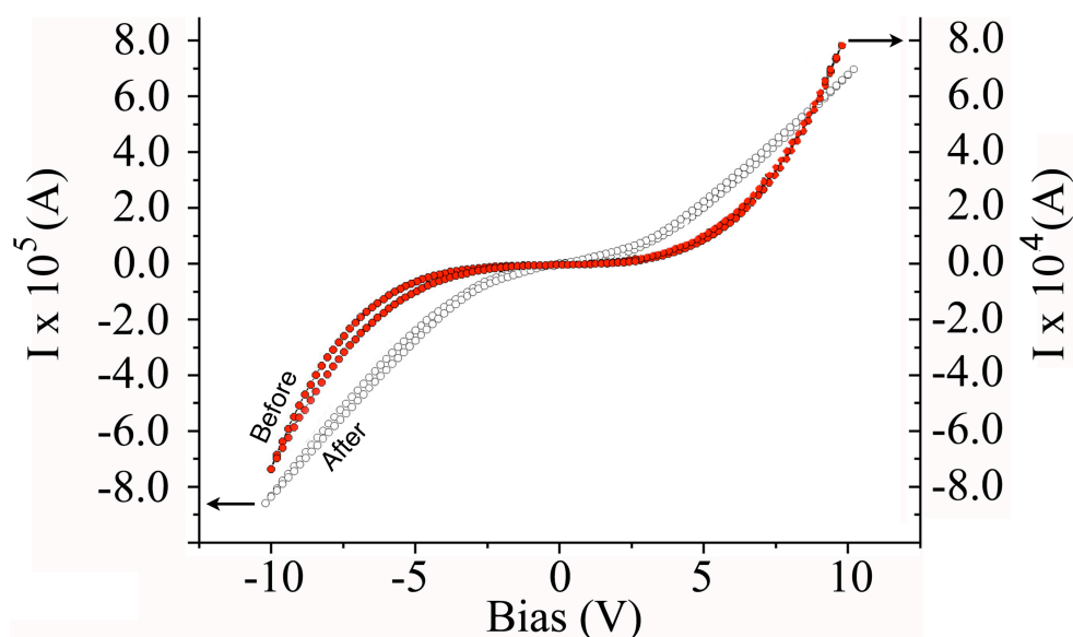
Figure 8. Room temperature I-V characteristics of the F16 MSDI device, before and after \text{NO}_x treatment.
