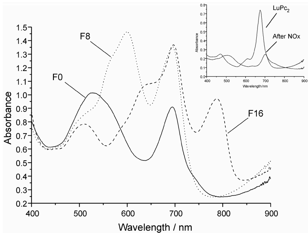
Figure 6. UV-vis. absorption spectra of the F0, F8 and F16 heterostructures deposited onto ITO, taken after the 30 min exposure to NO x vapors. The inset on the right displays UV-vis. absorption spectra of a LuPc 2 layer before and after undergoing the same experiment.
