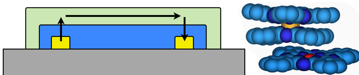
Figure 1. Left: Schematic side view of an MSDI heterojunction; the arrows indicate the main charges flow from one electrode to the other; Right: Compact mode view of mono- and bis-phthalocyanines.
