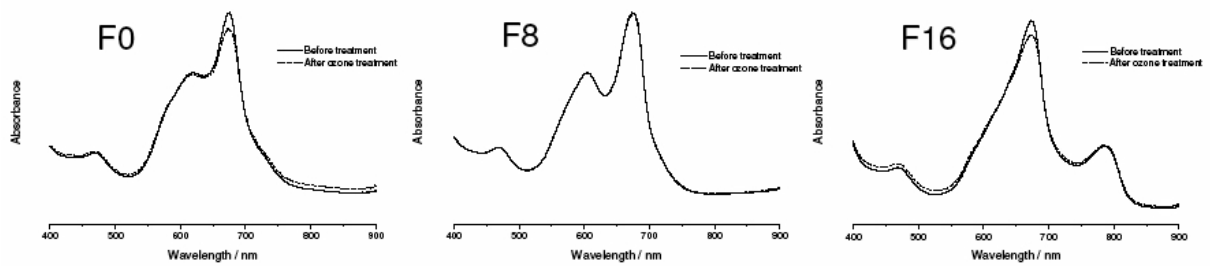
Figure 5. UV-vis absorption patterns of the heterostructures F0, F8 and F16 deposited on ITO glass substrates, after 50 min of exposure to high concentration of \text{O}_3 in air (1000 ppb, dotted line).
