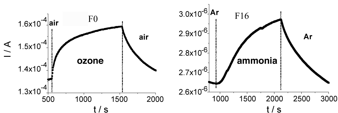
Figure 3. Typical sensing current response of F0 and F16 MSDIs when exposed, respectively, to 90 ppb of O 3 (alternately with pure air) and 35 ppm of NH 3 (alternating with argon).
