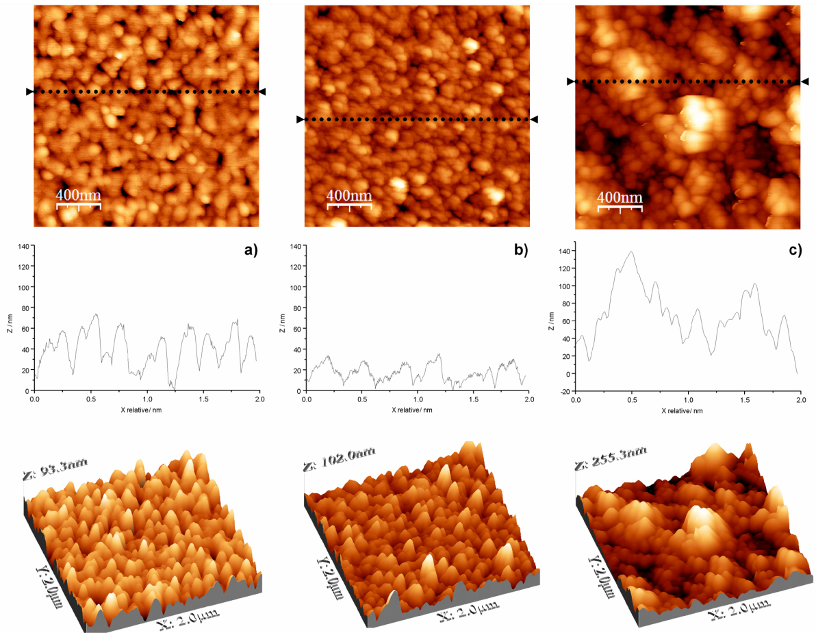
Figure 4. Typical TM-AFM images ( 2\ \mu\text{m} \times 2\ \mu\text{m} ) of the MSDI heterostructures. Relative height (Z) profiles as well as 3D representations are included. a) F0; b) F8; c) F16.
