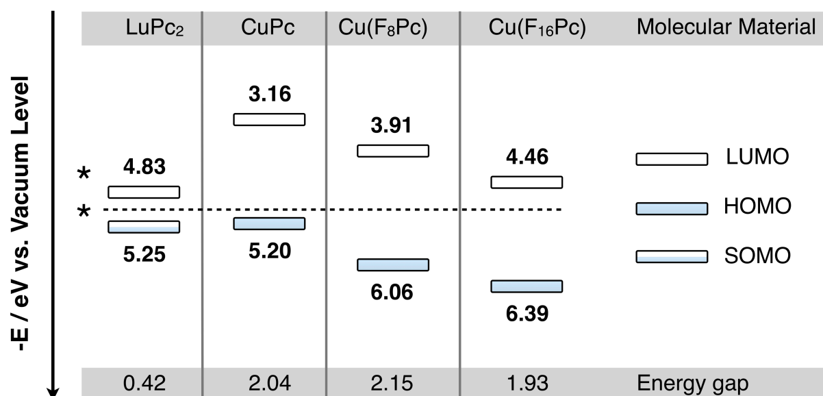
Figure 2. Scheme of the relative electron acceptor and donor energy levels (in eV) for all phthalocyanines derivatives used as molecular materials to form the MSDI displayed in this article. The values displayed on this figure have been estimated by means of cyclic voltammetry (*) in solution [12] and photoelectron spectroscopies [42].
