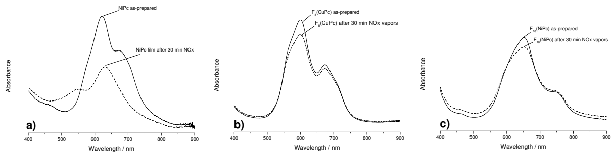
Figure 7. Evolution of the UV-vis. absorption patterns of some MPc single-layers after a 30 minute-long NO x vapour exposure.
