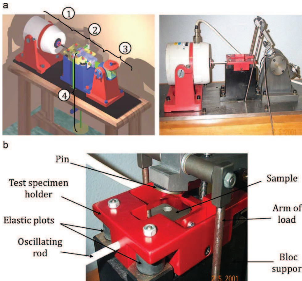
Fig. 3. Fretting device: (a) global view and (b) contact view.
