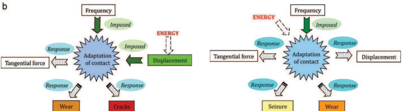
Fig. 1. Approach used for the damage analysis in fretting with a device which: (a) imposed tangential force and (b) imposed displacement.
