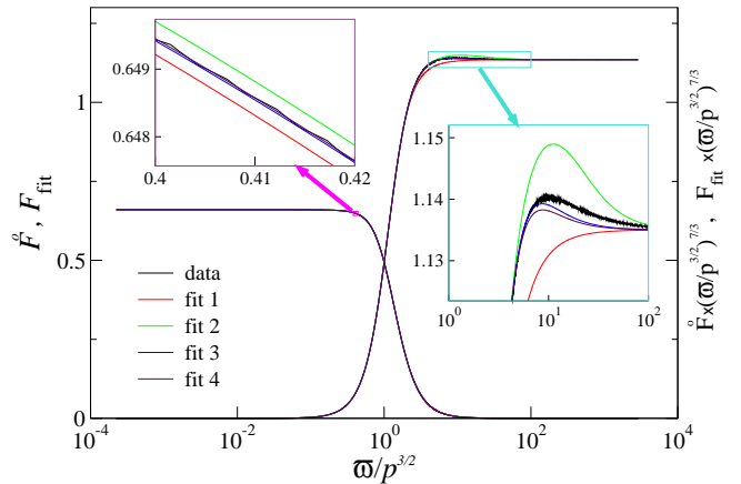
FIG. 4. (Color online) Illustration of the fitting procedure described in the text, using the same data for F as in Fig. 3 but with unified colors (black curves: on the left \mathring{F}(\tau) ; on the right \mathring{F}(\tau)\tau^{7/3} ). The four successive orders of the fit appear superimposed in the main graph; the two insets present large zooms (note the vertical scales) to differentiate them and highlight the convergence: the higher the order, the closer to the data (black-dotted curve) the fit lies. Note that for the right curve and inset \mathring{F}(\tau)\tau^{7/3} the differences are again magnified by a factor \tau^{7/3} .
