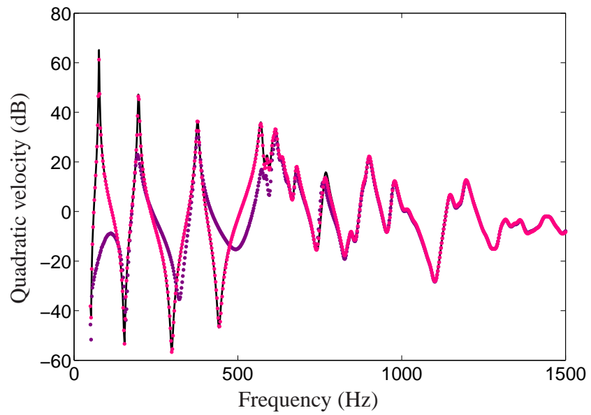
Figure 11: Frequency response function of a clamped sandwich structure whose left boundary (bottom skin only) is subjected to a uniform transverse force field: (—) FE reference solution; (•••) WFE solution with m = 33 wave modes selected by means of the error bound \mathcal{E}_s ; (•••) WFE solution with m = 63 wave modes selected by means of the error bound \mathcal{E}_s .
