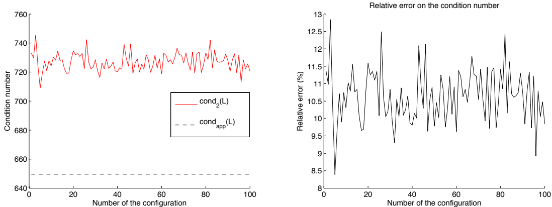
(a) Comparison between the exact and approximate (b) Relative error on the condition number (%) (see condition numbers relation (36))
