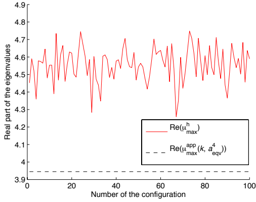
(a) Comparison between the real part of the largest eigenvalue and its estimate (b) Comparison between the imaginary part of the largest eigenvalue and its estimate
