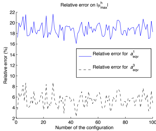
(e) Relative error on the modulus of \mu_{max}
