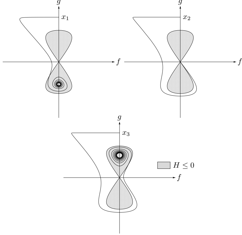
FIGURE 2. x_1 \in A_1 , x_2 \in I_1 , x_3 \in A_2
