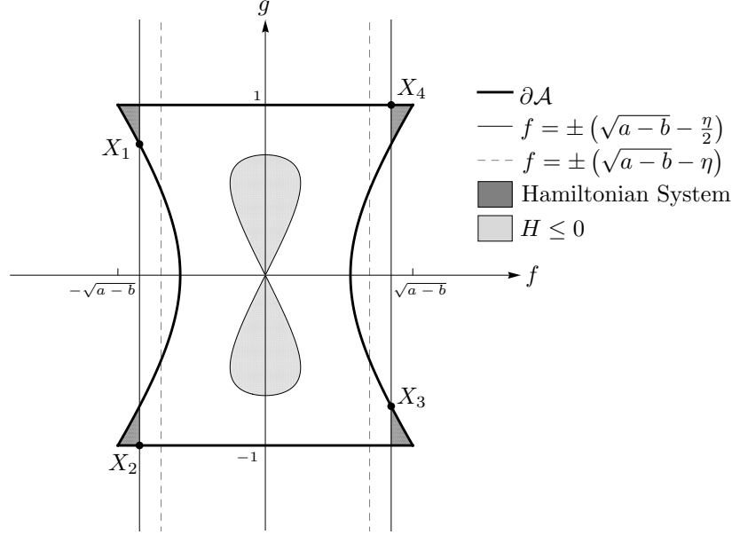
FIGURE 1. Regularized System
