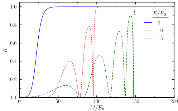
FIG. 2 (color online). Reflection probability R as a function of the normalized magnetic field M for various Fermi energies E , and \alpha_0 / v_F = 0.1 . The energy unit is E_0 = \hbar v_F / d .
