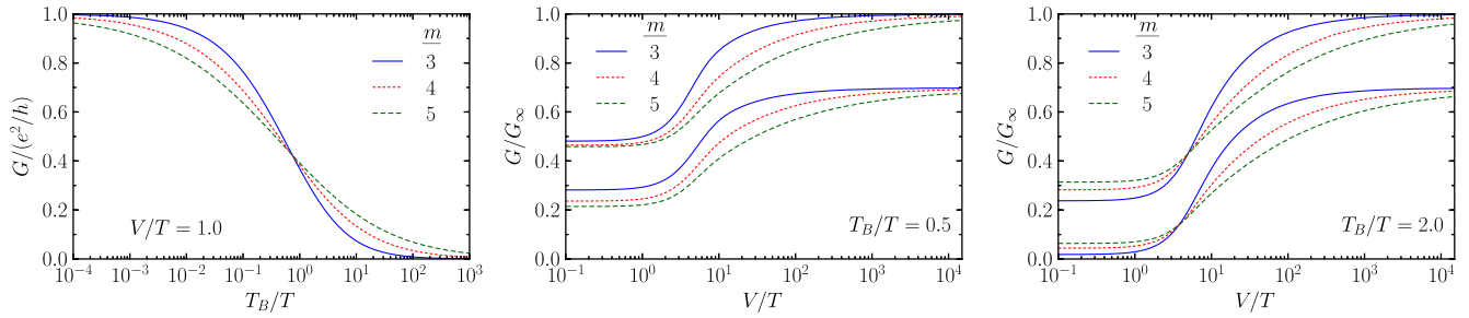
FIG. 3 (color online). Differential conductance for different values of g = 1 - 1/m . Left figure: G = dI/dV (with contact corrections) as a function of T_B/T . Right figures: G = dI/dV as a function of V/T for two different values of T_B/T . The differential conductance has been scaled with the value G_\infty = e^2/h and (1 - 1/m)e^2/h with and without contact corrections, respectively. The curves without contact corrections have been shifted down by 0.3 for clarity.
