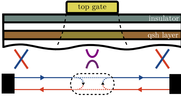
FIG. 1 (color online). Proposed experimental setup. A top gate is used to locally tune the strength of the Rashba spin-orbit coupling. Combined with a magnetic field, a local energy gap in the edge spectrum generates backscattering.
