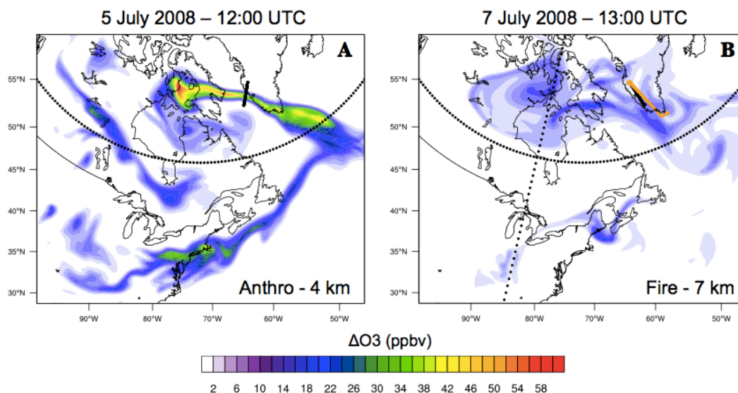
Fig. 11. Maps of enhancements in ozone in anthropogenic and fire plumes ( \Delta O_3 ) demonstrating the spatial extent of plumes sampled by the ATR-72 and Falcon-20 on 5 and 7 July 2008. The ATR-42 aircraft flight tracks are in black and the Falcon-20 flight track is in orange. For anthropogenic plumes, the latitude 55^\circ N that is used to define fresh ( <2 km, \text{lat} < 55^\circ N ) and aged ( \text{lat} > 55^\circ N ) anthropogenic plumes is indicated by the dotted black line. For fire plumes, the latitude 55^\circ N longitude 85^\circ W (used to define aged fire plumes) are indicated by dotted black lines. These same plumes are shown as enhanced CO mixing ratios in Fig. 2, panel (d) for the anthropogenic emissions and panel (e) for fires.
