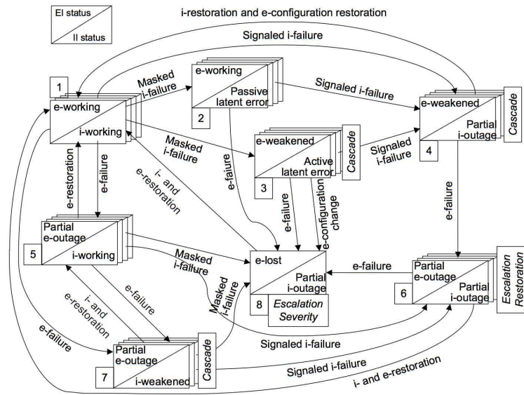
Fig. 1. Model of the two infrastructures when considering accidental failures.
