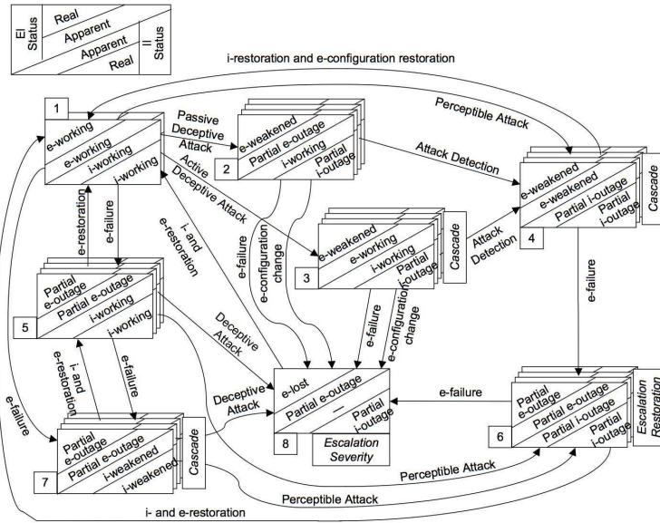
Fig. 2. Model of the two infrastructures when considering malicious attacks.
