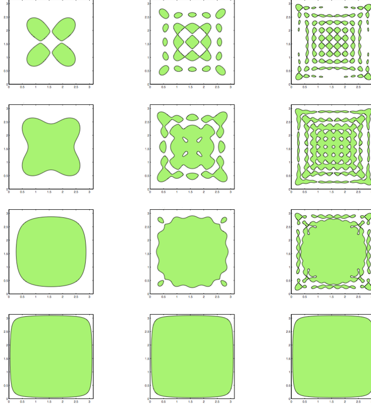
Figure 5: \Omega = (0, \pi)^2 , with Dirichlet boundary conditions. Row 1: L = 0.2 ; row 2: L = 0.4 ; row 3: L = 0.6 ; row 4: L = 0.9 . From left to right: N = 2 (4 eigenmodes), N = 5 (25 eigenmodes), N = 10 (100 eigenmodes).
