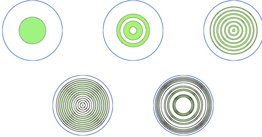
Figure 4: \Omega = \{x \in \mathbb{R}^2 \mid |x| \leq 1\} , with Dirichlet boundary conditions, and L = 0.2 . Optimal domain for N = 1 (1 eigenmode), N = 2 (4 eigenmodes), N = 5 (25 eigenmodes), N = 10 (100 eigenmodes) and N = 20 (400 eigenmodes).
