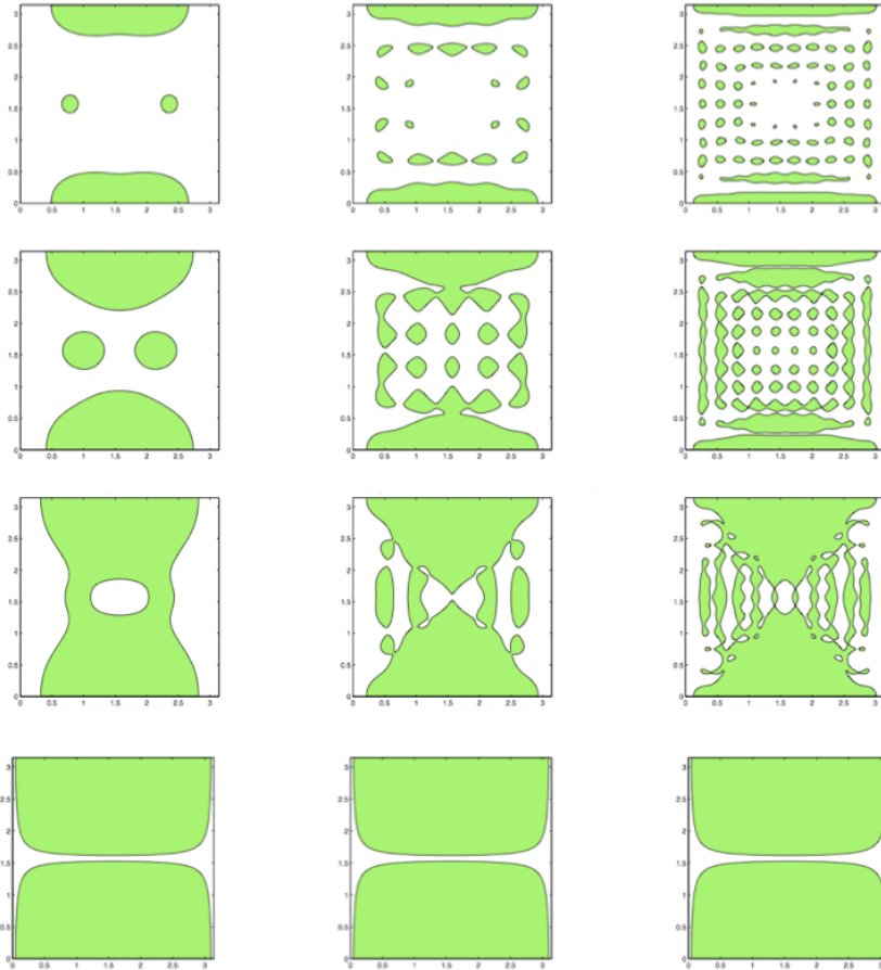
Figure 7: \Omega = (0, \pi)^2 , with Dirichlet boundary conditions on \partial\Omega \cap (\{x_2 = 0\} \cup \{x_2 = \pi\}) and Neumann boundary conditions on the rest of the boundary. Row 1: L = 0.2 ; row 2: L = 0.4 ; row 3: L = 0.6 ; row 4: L = 0.9 . From left to right: N = 2 (4 eigenmodes), N = 5 (25 eigenmodes), N = 10 (100 eigenmodes).
