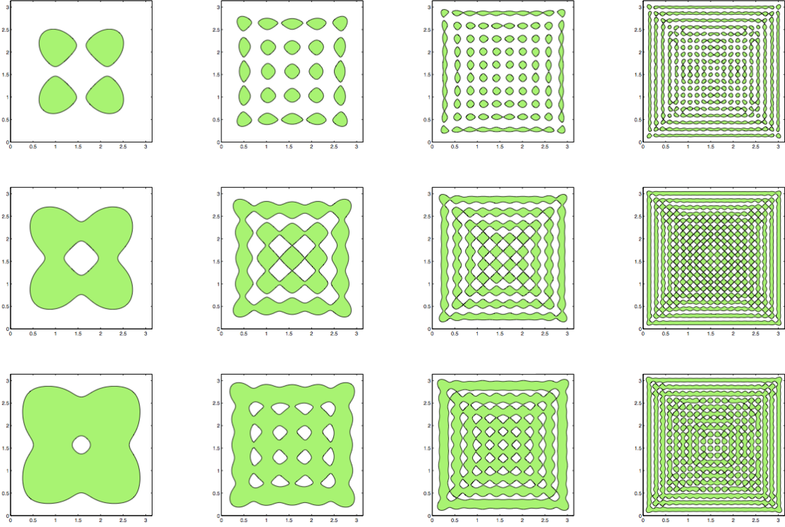
Figure 3: \Omega = (0, \pi)^2 , with Dirichlet boundary conditions. Row 1: L = 0.2 ; row 2: L = 0.4 ; row 3: L = 0.6 . From left to right: N = 2 (4 eigenmodes), N = 5 (25 eigenmodes), N = 10 (100 eigenmodes), N = 20 (400 eigenmodes). The optimal domain is in green.
