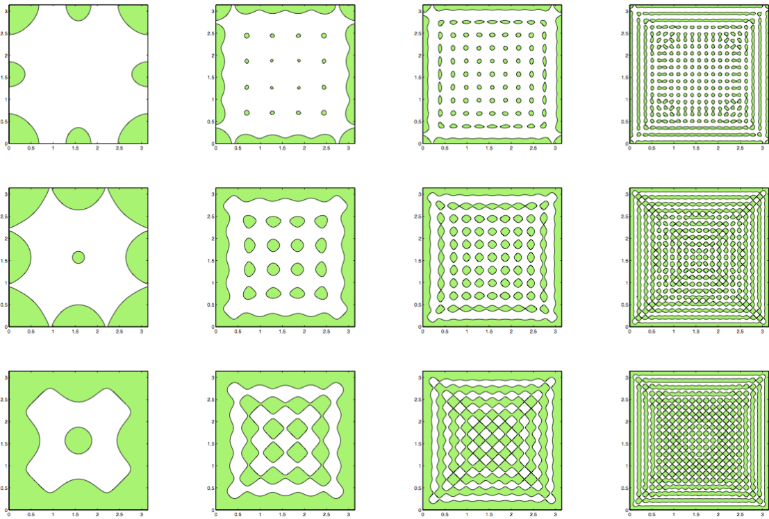
Figure 6: \Omega = (0, \pi)^2 , with Neumann boundary conditions. Row 1: L = 0.2 ; row 2: L = 0.4 ; row 3: L = 0.6 . From left to right: N = 2 (4 eigenmodes), N = 5 (25 eigenmodes), N = 10 (100 eigenmodes), N = 20 (400 eigenmodes).
