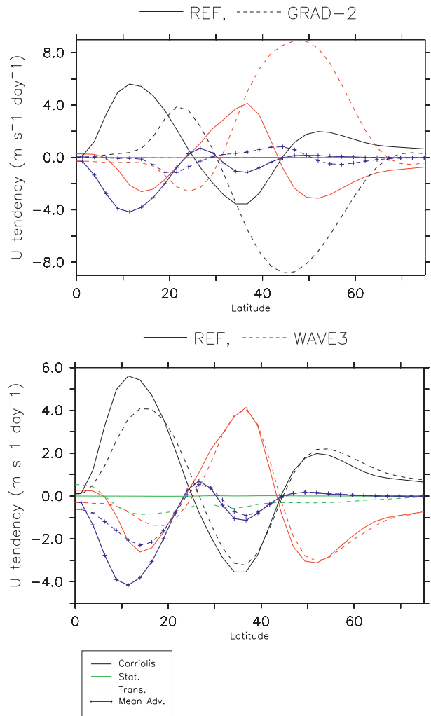
FIG. 10. Zonal-mean zonal wind balance at the 200-hPa height and the contribution to wind tendency ( \text{m s}^{-1} \text{day}^{-1} ) from the mean advection, Coriolis torque, and stationary and transient eddies. The continuous lines designate the results for the simulation REF; dashed lines indicate the results of the simulations (top) GRAD-2 and (bottom) WAVE3.
