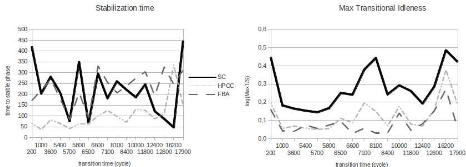
Fig. 8. Compared transitional performances during the 20000 cycles scenario.
