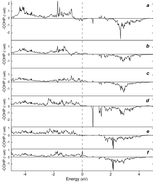
Figure 7. COHP curves for Mo-Mo bonds: (a) 2.680 Å, (b) 2.712 Å, (c) 2.808 Å, (d) 2.674 Å, (e) 2.686 Å, (f) 2.772 Å computed for \text{In}_2\text{Mo}_{15}\text{Se}_{19} . (a–d) and (e–f) curves correspond to Mo-Mo bonds of \text{Mo}_9 and \text{Mo}_6 motifs, respectively.
