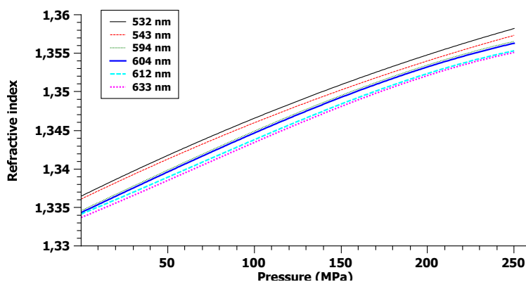
Fig 2. Refractive index as a function of pressure for various wavelengths
