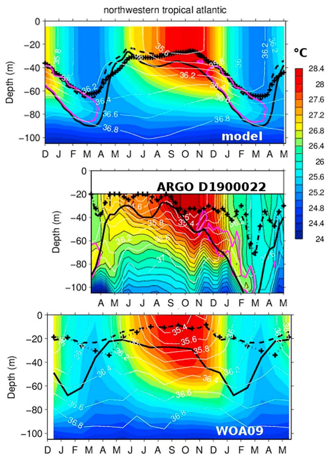
Figure 3. (top) Time evolution of temperature (colors, in ^{\circ}\text{C} ) and salinity (white contours, in psu) from the surface to 100 m depth averaged over the thick box in the northwestern tropical Atlantic shown in Figure 2. The thick black lines shows the depth D_{T^*-0.2} (solid), the MLD (dashed) and the halocline depth D_{S^*+\Delta S} with \Delta S = 0.06 psu diagnosed from the model data averaged over the same area (crosses). The magenta contour highlights vertical temperature inversions of 0.2^{\circ} and more. (middle) Time evolution of temperature (colors) and salinity (white contours) from the surface to 100 m depth of the ARGO float D1900022 that traveled in the same area (between 55.5 and 60^{\circ}\text{W} and 14 and 22^{\circ}\text{N} between April 2002 and May 2003). A running mean over 3 points with equal weights has been applied to all time series. (bottom) Same as Figure 3 (top) using the monthly mean temperature and salinity fields from WOA09 [Locarnini et al., 2010; Antonov et al., 2010].
