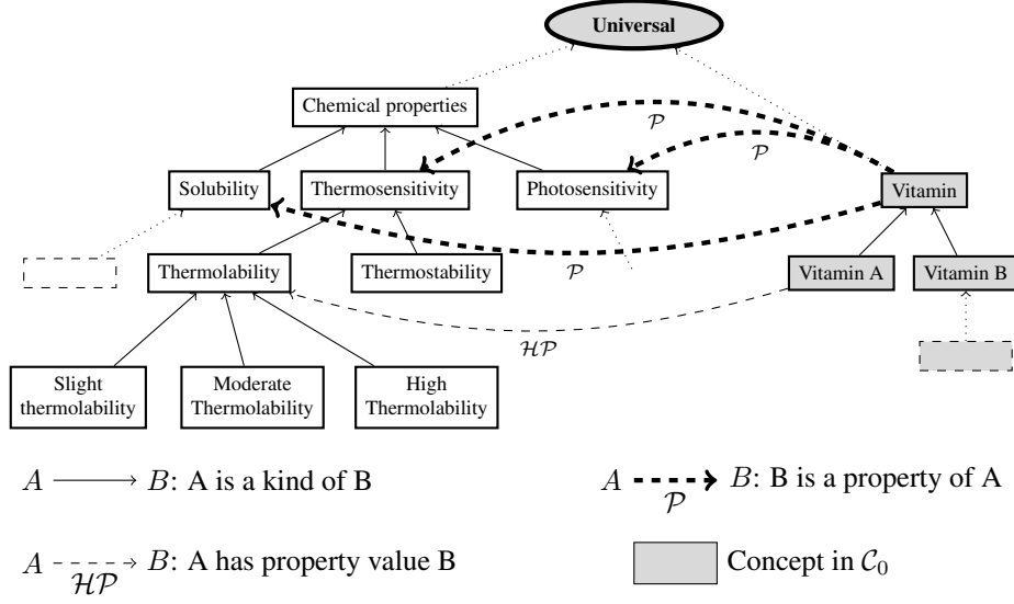
Figure 6: Excerpt of concept and relation additions to \Omega_0 .
