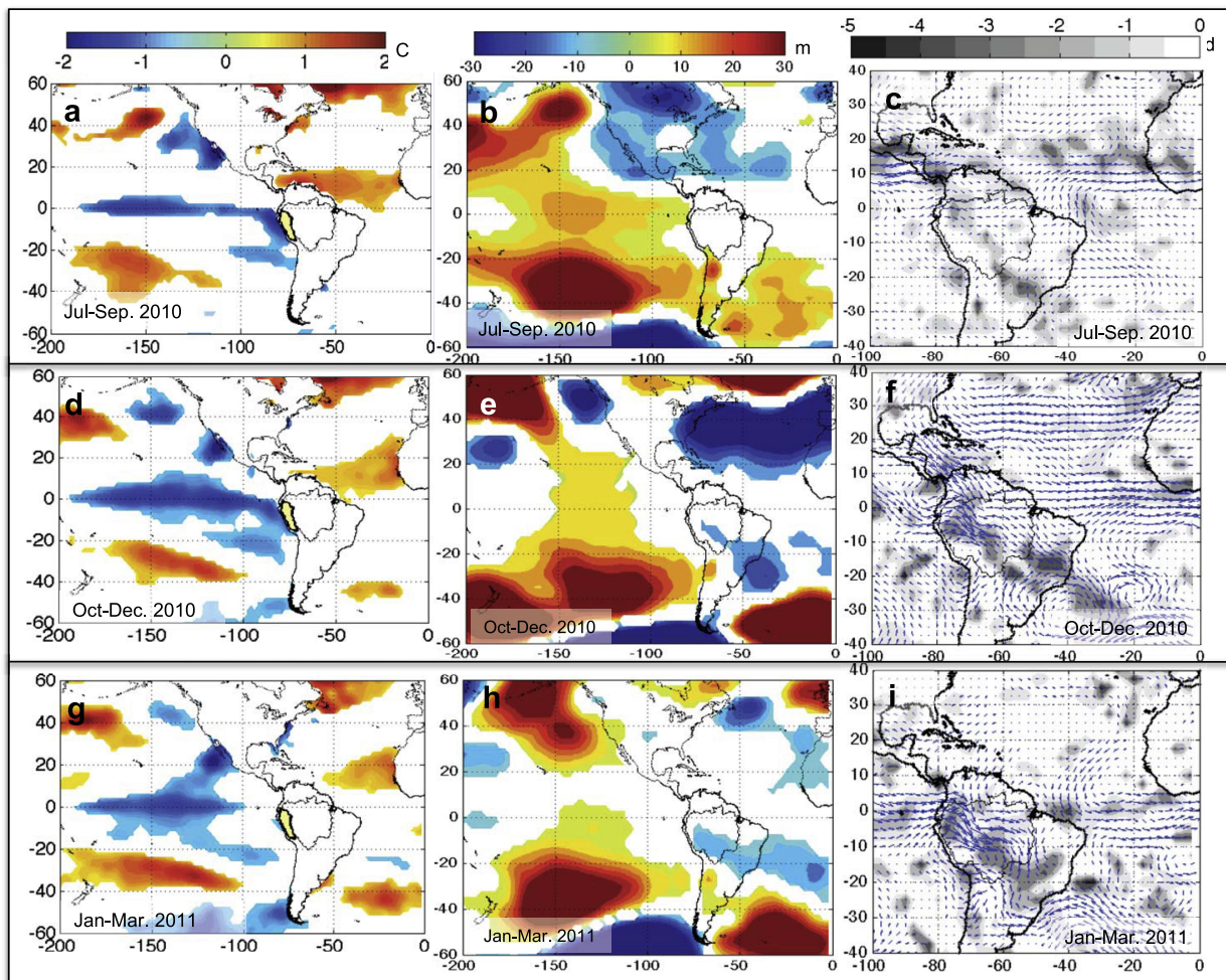
Figure 3. SST (°C, left), 850 hPa geopotential height (m, center), vertically integrated water vapor flux anomalies (vectors, kg m -1 day -1 , right) and negative divergence standardized values (contours, without unit) between the ground and 300 hPa (right) in (a)–(c) July–August–September 2010, (d)–(f) October–November–December 2010, (g)–(i) January–February–March 2011. Only values higher than 1 × standard deviation are plotted (2 × standard deviation for SST data).
