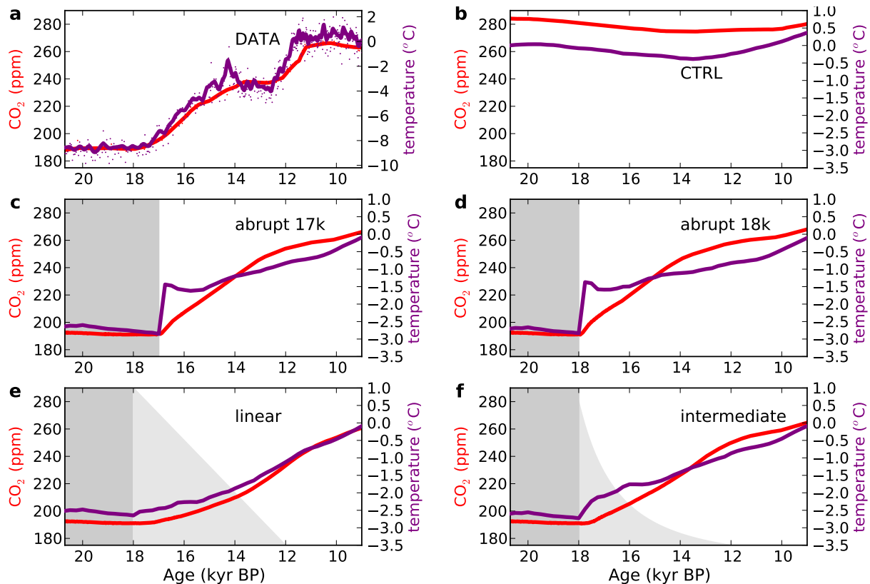
Fig. 16. Evolution of CO 2 (ppm) and Antarctic temperature (°C) during the deglaciations for (a) the data (Monnin et al., 2001; Lourdantou et al., 2010; Jouzel et al., 2007), (b) the CTRL simulation (with carbonate compensation), (c, d, e, f) the simulations with interactive diffusion, iron fertilization and different brines scenarios as defined in Fig. 14a. The grey shading indicates the evolution of the sinking of brines according to each scenario.
