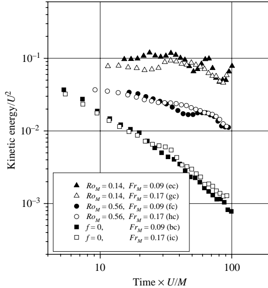
FIGURE 4. Decay of mean kinetic energy for several parameters. The initial Reynolds number is the same for the different experiments, Re_M = 9000 .
