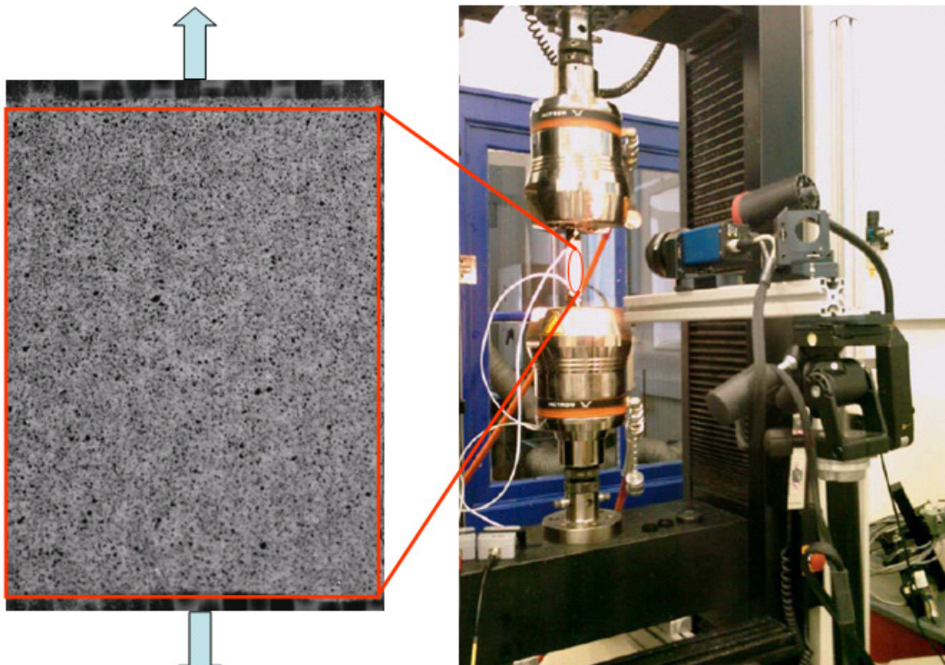
Figure 1. Specimen with DIC pattern and experimental setup.
