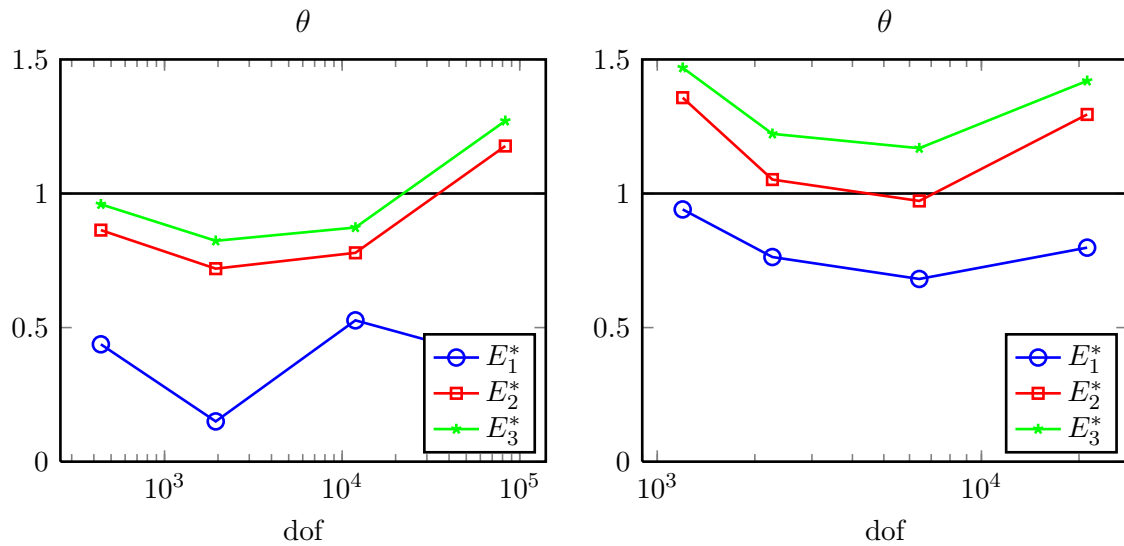
Figure 10: Example 4: L-Shape. Effectivity index. Q4 (left) and Q8 (right).
