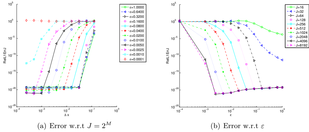
Figure 11: \text{err}_{J\epsilon}(t = 0.13) for time splitting scheme
