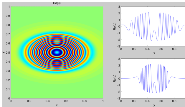
Figure 22: \text{Re}(u^\varepsilon)(t = 0.035)
