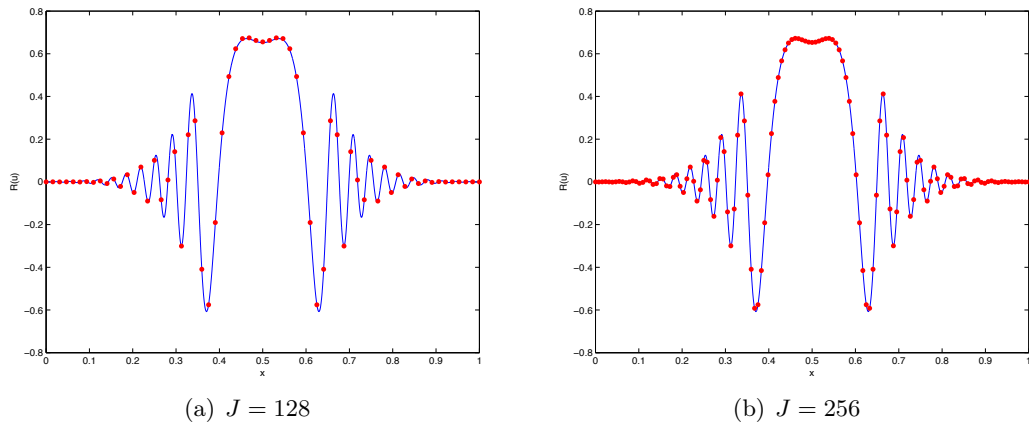
Figure 12: \text{Re}(u^\epsilon) at T = 0.05 for \epsilon = 0.005
