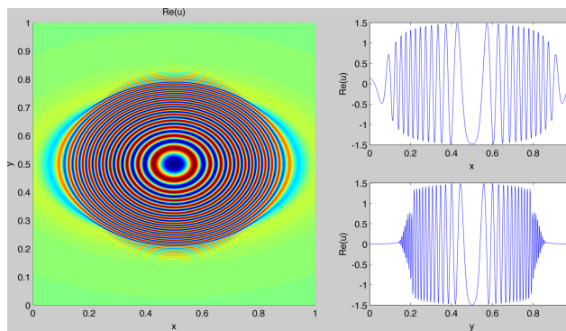
Figure 23: \text{Re}(u^\varepsilon)(t = 0.08)
