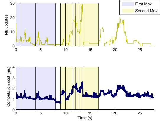
Fig. 27: Experiment B: Number of algorithm iterations and computation time when using the projected cascade described in [De Lasa et al., 2010].
