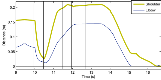
Fig. 21: Experiment B-2: Distance to the obstacle.
