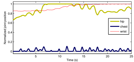
Fig. 5: Walking with an umbrella: normalized positions of some typical joints. The joint limits are respected at any time.
