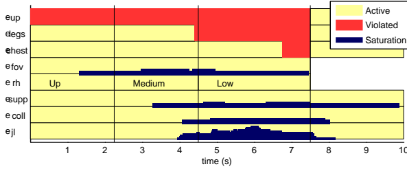
Fig. 29: Experiment C: Task sequence.
