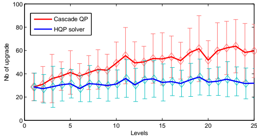
Fig. 5: Number of activations and deactivations using a cascade of QP and a our solver for the same problems as in Fig. 4. The number increases with p for the cascade of QP and remains constant for the HQP solver.
