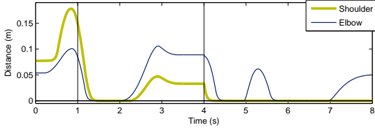
Fig. 18: Experiment B-1: distance to the obstacle during the first movement. The obstacle is on the way between the left-arm initial position and the wheel: the two constraints of the shoulder and the elbow become active at T = 1.1s and T = 1.2s . They are deactivated later during the grasping phase, at T = 2s and T = 2.1s . At each loop of the wheel, the left arm comes close to the obstacle, between T = 4s and T = 5s , and a second time between T = 5.7s and T = 7s .
