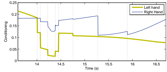
Fig. 24: Experiment B-2: Conditioning number of the hand tasks when both hands are moving the wheel. The vertical dot lines show the inequality activations. The conditioning number evolves both continuously with the changes in the Jacobians and discreetly at each constraint activation.
