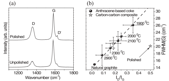
FIG. 3. (a) Raman spectra of polished and unpolished carbon-carbon composite collected using the laser energy 2.41 eV. (b) The I_D/I_G and FWHM(G) values of the unpolished anthracene-based coke treated at different temperatures (filled circles) and carbon-carbon composite (opened stars) both polished and unpolished.
