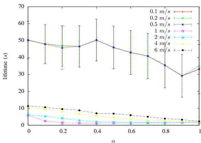
Fig. 7. Life time of cluster head status according to \alpha and the speed
