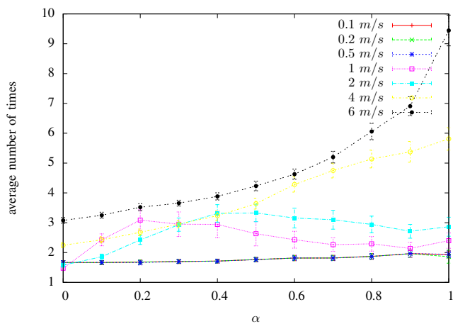
Fig. 6. Number of times a node became head of a cluster according to \alpha and the speed
