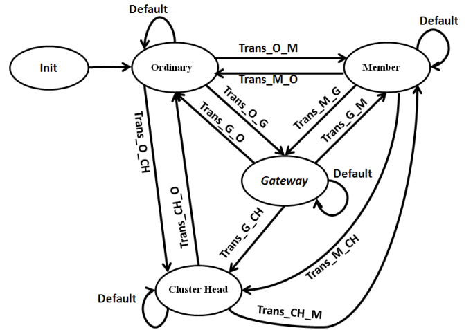
Fig. 2. Finite state machine of the clustering process
