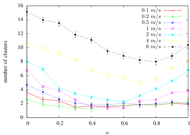
Fig. 8. Number of clusters according to \alpha and the speed
