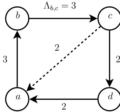
Figure 7: Bang-bang policies are suboptimal even when the number of vehicles tends to infinity.
