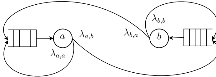
Figure 3: A closed queuing network model: servers represent users demands.
