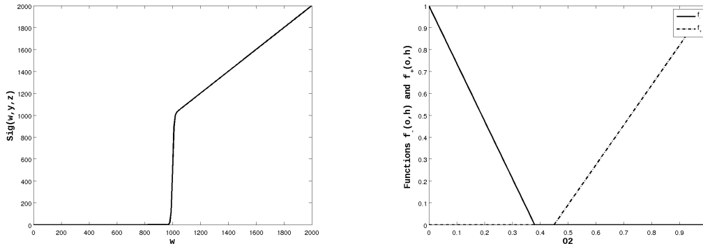
FIGURE 2. (Left) . Graph of the function w \mapsto \text{Sig}(w, y, z) with y = r_{Ang, EC} and z = s_{Ang, EC} . (Right) . Graph of the functions o \mapsto f_-(o, h) with h = h_{PQ} and o \mapsto f_+(o, h) with h = h_{QP} .
