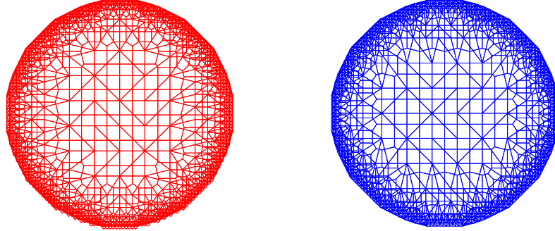
Figure 6: The Delaunay triangulation and the Voronoi cells (left: horizontal velocity, right: vertical velocity).
