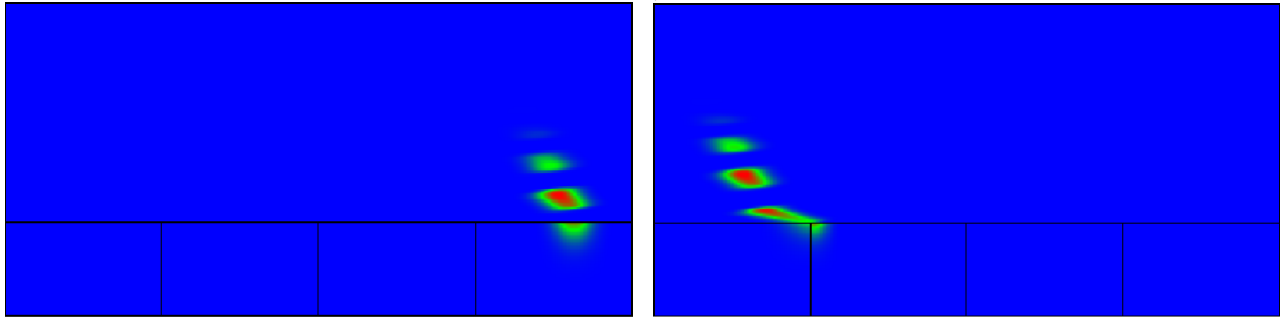
b) t = 2.58 , cell cycles 3 – 4 transition \Omega_2^3 \rightarrow \Omega_1^4 and \Omega_1^4 \not\rightarrow \Omega_3 . \phi_{max} = 430
