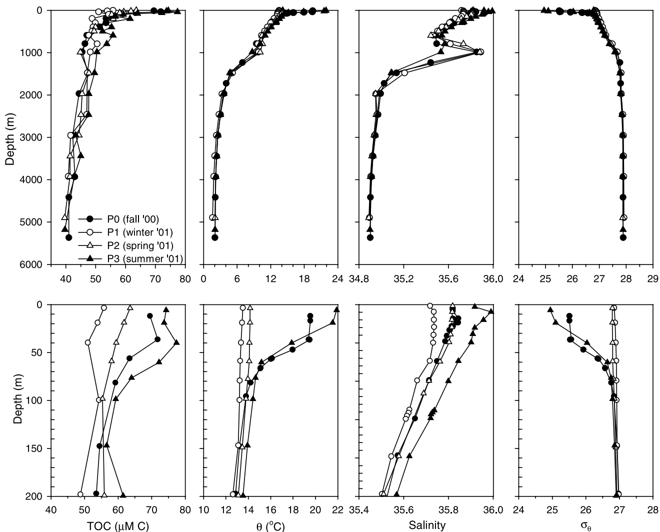
Figure 2. (top) Full-depth profiles of TOC, potential temperature ( \theta ), salinity, and potential density anomaly ( \sigma_{\theta} ) at 41.5^{\circ}\text{N} , 18^{\circ}\text{W} in each POMME cruise and (bottom) the corresponding profiles in the upper 200 m.
