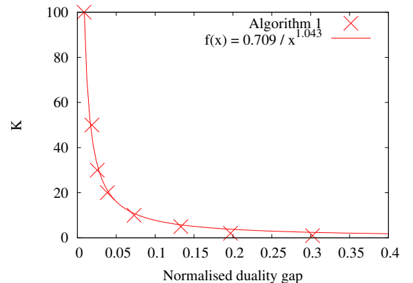
Figure 4: K parameter against the resulting mean normalized gap value for Algorithm 1 on ADULT.
