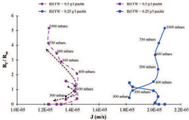
Fig. 10. Pectin's impact on reversible R_{rf} (■) and irreversible R_{ir} (●) fouling.
