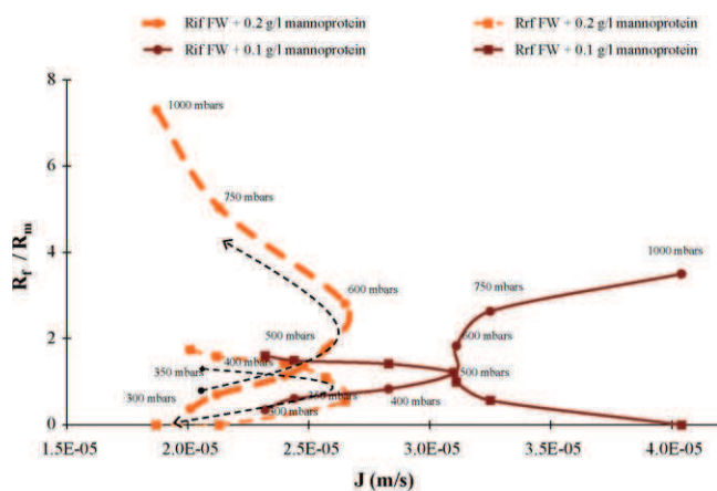
Fig. 11. Mannoproteins' impact on reversible R_{rf} (■) and irreversible R_{ir} (●) fouling.
