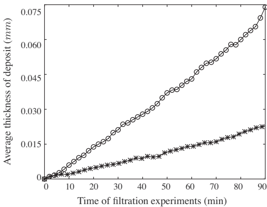
Fig. 11. The temporal evolution of the average thickness of particle deposit: -- \phi = 10^{-3} v/v; q = 2 ml h -1 (dispersed in ultra-pure water), and -- \phi = 10^{-3} v/v; q = 2 ml h -1 (dispersed in KCl at 10^{-1} M).
