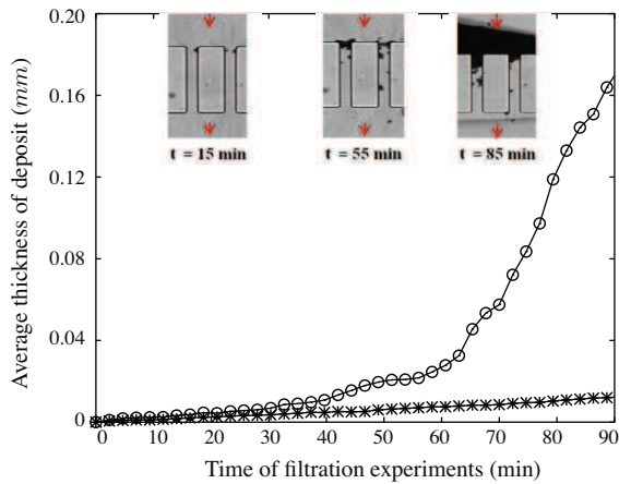
Fig. 5. The temporal evolution of the average thickness of particle deposit: -\ast- \phi = 10^{-3} v/v; q = 2 ml h ^{-1} , and -o- \phi = 5.10^{-3} v/v; q = 2 ml h ^{-1} (dispersed in ultra-pure water) with snapshots of the cluster formation at t = 15, 55 and 85 min.
