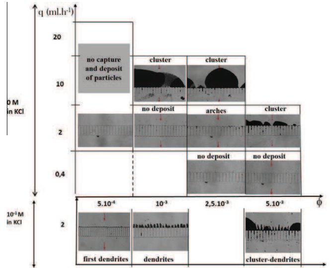
Fig. 12. Summary of different deposit structures of latex particles formed during filtration experiments. For q \leq 2 ml h -1 , images are taken after 90 min of filtration while experiments performed at q = 10 ml h -1 last only 40 min.
