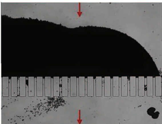
Fig. 6. \phi = 10^{-3} v/v; q = 10 ml h ^{-1} : cluster formation after 40 min of dead-end filtration. Latex suspensions are dispersed in ultra-pure water.
