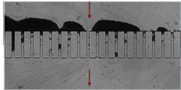
Fig. 4. \phi = 5 \cdot 10^{-3} \text{ v/v} ; q = 2 \text{ ml h}^{-1} : cluster formation after 90 min of dead-end filtration. Latex suspensions are dispersed in ultra-pure water.
