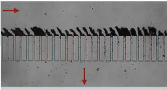
Fig. 10. \phi = 10^{-3} v/v; q = 2 ml h -1 : formation of tilted dendrites after 90 min of cross-flow filtration. Latex particles are dispersed in KCl-water solution at 10^{-1} M.
