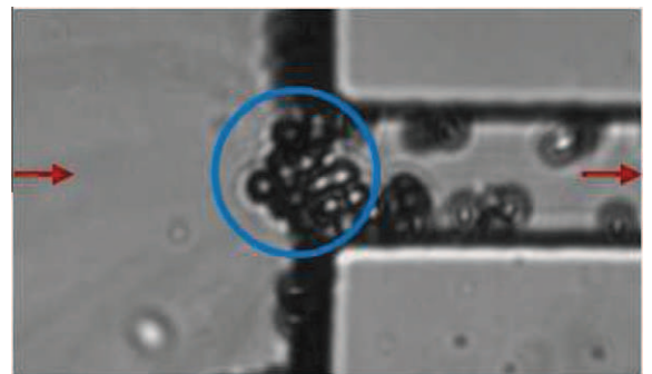
Fig. 16. Final state of the bridging mechanism after the passage of 7650 particles through the micropore in 5 s: close-up on particles blocking the microchannel entrance after 35 min of dead-end filtration ( \phi = 5 \times 10^{-3} ; q = 2 \text{ ml h}^{-1} ).
