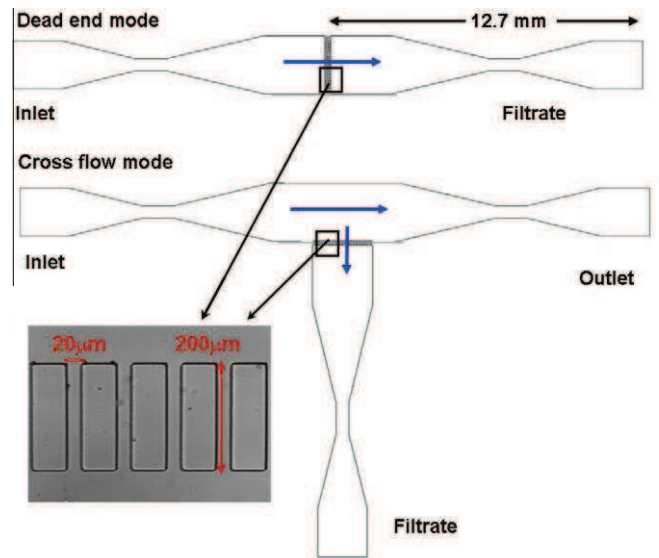
Fig. 1. Schematic view of the PDMS micro-separators used for dead-end and cross-flow filtration.
