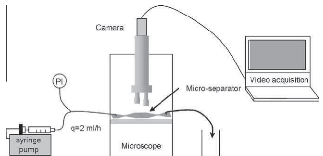
Fig. 2. Experimental set-up for imaging the channel blockage.
