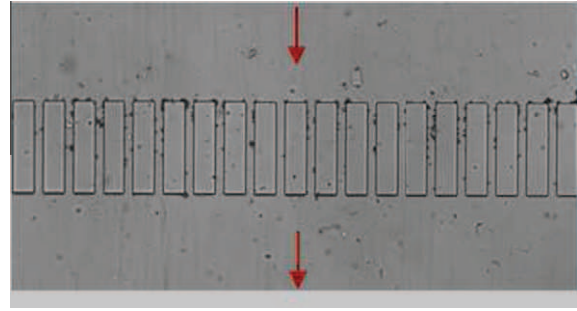
Fig. 3. \phi = 10^{-3} \text{ v/v} ; q = 2 \text{ ml h}^{-1} : no deposit of particles after 90 min of dead-end filtration. Latex suspensions are dispersed in ultra-pure water.
