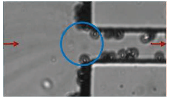
Fig. 15. Close-up on the open microchannel entrance after 34 min and 55 s of dead-end filtration ( \phi = 5 \times 10^{-3} ; q = 2 \text{ ml h}^{-1} ).
