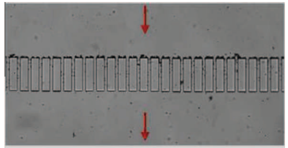
Fig. 8. \phi = 5.10^{-4} v/v; q = 2 ml h ^{-1} : early instants of dendrites formation after 90 min of dead-end filtration. Latex suspensions are dispersed in KCl-water solution at 10^{-1} M.
