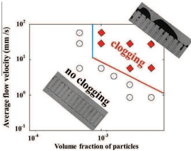
Fig. 13. Experimental conditions leading to deposition of latex particles and to the microsystem clogging. Results shown in this figure represent the state of microsystem after 90 min of filtration performed by dispersing the latex particles in ultra-pure water and varying the volume fraction of particles and the average flow velocity: filled diamonds: clogging, open circles: no clogging.
