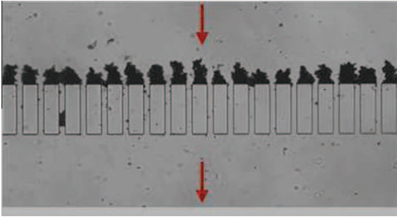
Fig. 9. \phi = 10^{-3} v/v; q = 2 ml h -1 : formation of straight dendrites after 90 min of dead-end filtration. Latex particles are dispersed in KCl-water solution at 10^{-1} M.
