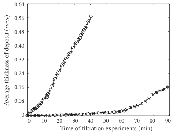
Fig. 7. The temporal evolution of the average thickness of particle deposit: -\ast- \phi = 5.10^{-3} v/v; q = 2 ml h ^{-1} , and -o- \phi = 10^{-3} v/v; q = 10 ml h ^{-1} (dispersed in ultra-pure water).
