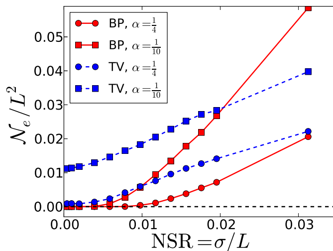
Figure 7. Fraction or error \mathcal{N}_e/L^2 vs. normalized measure noise \sigma/L , for BP-tomo and the convex algorithm (TV). These numerical tests have been performed for two different undersampling rates \alpha . For a small noise, BP-tomo always outperforms the convex algorithm. In particular, there is a finite interval of noise intensity for which the reconstruction is error-free.
