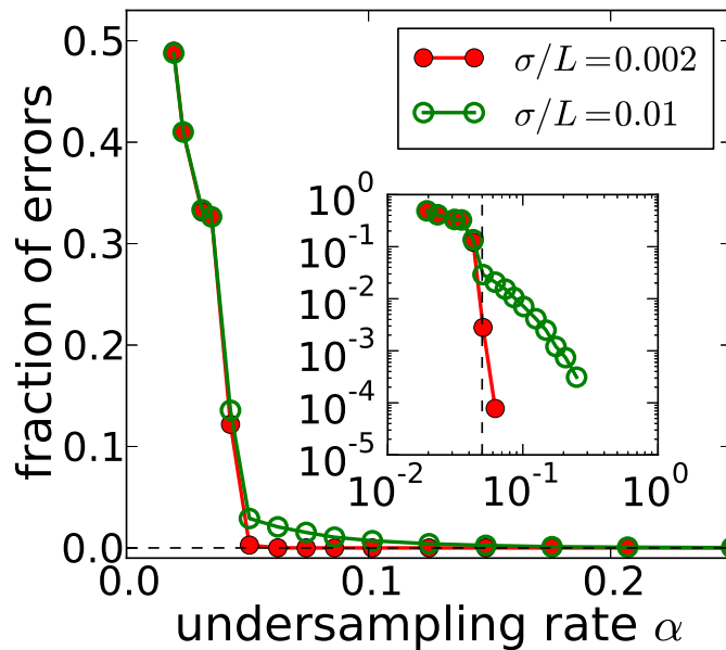
Figure 10. Fraction of error \mathcal{N}_e/L^2 as a function of the measurement rate \alpha , for BP-tomo and two different values of the noise amplitude (inset in log-log coordinates). The transition is sharper for a small noise. In the inset, the dashed vertical line represents the empirical value of the noise-free critical undersampling rate.
