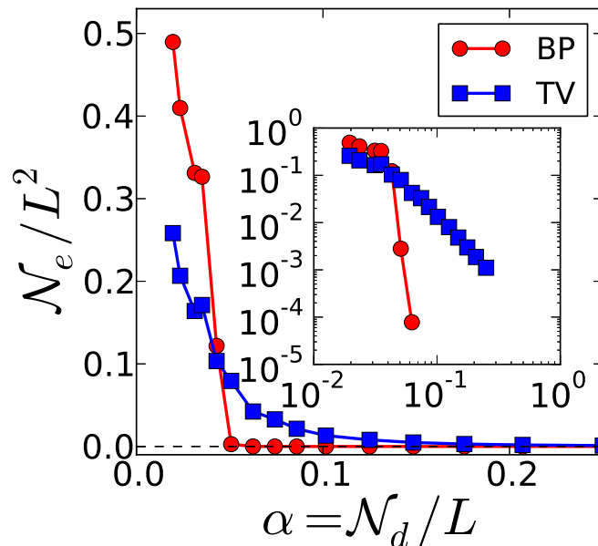
Figure 9. Fraction of error \mathcal{N}_e/L^2 as a function of the measurement rate \alpha , for BP-tomo and the convex algorithm (TV) (inset in log-log coordinates). These numerical tests have been performed for a small noise \sigma/L = 0.002 . For both algorithms, the number of errors decrease when the measurement rate is increased, but the evolution is very different. For BP-tomo, the evolution is very sharp: above a certain threshold, the reconstruction is error-free. However, below this threshold the number of errors displays a sharp transition and converges quickly to the value for a random image (50 % of errors). The convex algorithm fares better below the BP-tomo threshold, but does not have a "phase transition", so that it is outperformed by BP above the threshold.
