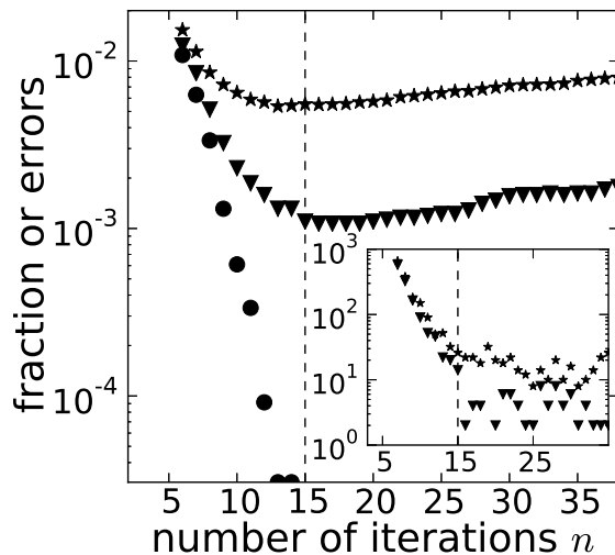
Figure 6. Stop criterion in the noisy case - Main axes: fraction of error compared to ground truth vs. number of iterations n for a signal to noise ratio of 0.6 % ( \bullet ), 1 % ( \blacktriangledown ) and 2 % ( \star ). For a small amplitude of the noise, the number of errors converges to zero (SNR = 0.6%). For a large amplitude of the noise, the fraction of errors reaches a minimum after the number of iterations needed to reach an exact reconstruction for a smaller value of the noise (here, n = 15 ). Inset: number of flipped spins between two iterations vs. number of iterations. We observe that the minimum fraction or errors correlates well with a change of slope for the number of flipped spins.
