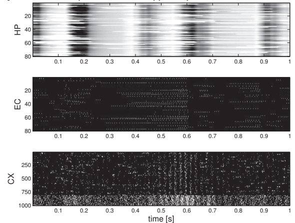
Fig. 7. Memory consolidation in the cortical map. Memory retention is estimated from the signal per noise ratio between the hippocampal items and the cortical map activity with the Victor and Purpura distance between two spike trains [30]. The cortical map learns the hippocampal patterns at a very slow rate compared with the hippocampus.
