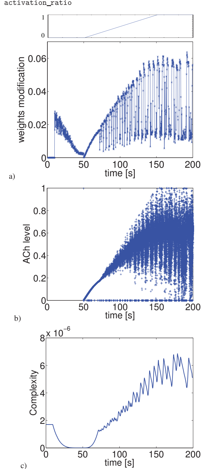
Fig. 4. Weight modification for Hebbian learning with gradual activation of ACh modulation starting at t = 50sec resp. a) and b). Complexity measures computed from the connection matrix of the hippocampal network relative to cholinergic activation rate (c).
