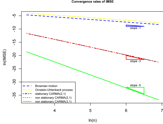
FIGURE 3.5. Logarithm of e_1^2(\text{app}(\hat{r}_0)) , i.e. the IMSE in function of \ln(n) , for different type of processes. The dashed line correspond to Brownian motion, long dashed line to O.U., dashed line to non stationary CARMA(2,1), dotted-dashed line to stationary CARMA(2,1) and solid line to non stationary CARMA(3,1). The small triangles near lines are here to indicate the theoretic slope.
