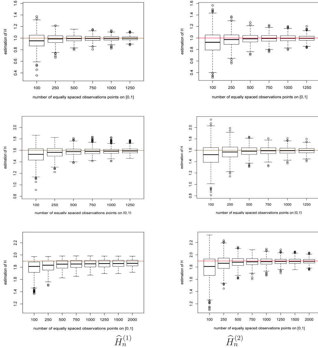
FIGURE 3.1. Each boxplot correspond to 1000 estimation of H by \widehat{H}_n^{(1)} on the left and \widehat{H}_n^{(2)} on the right of the graph. Each realization consists in n equally spaced observations on [0, 1] of a fBm with \beta_0 = 0.5 (top), \beta_0 = 0.8 (middle), \beta_0 = 0.95 (bottom), where n = 100, 250, 500, 750, 1000, 1250, 1500, 2000 .
