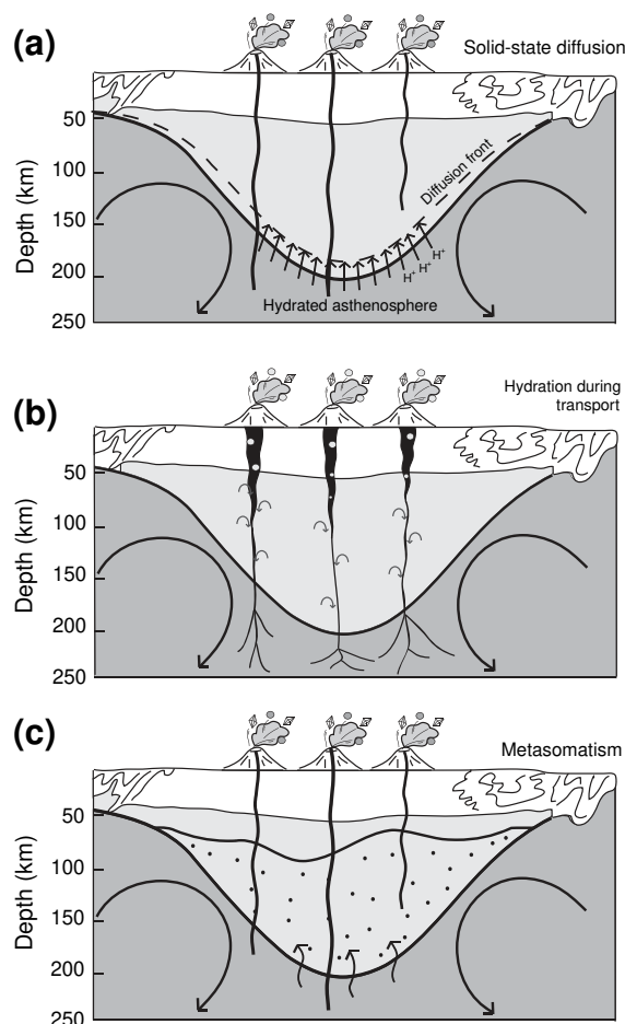
Fig. 14. Sketches illustrating the three scenarii proposed to explain the variation of \text{OH}^- concentration in olivine with depth in the Kaapvaal craton root.
