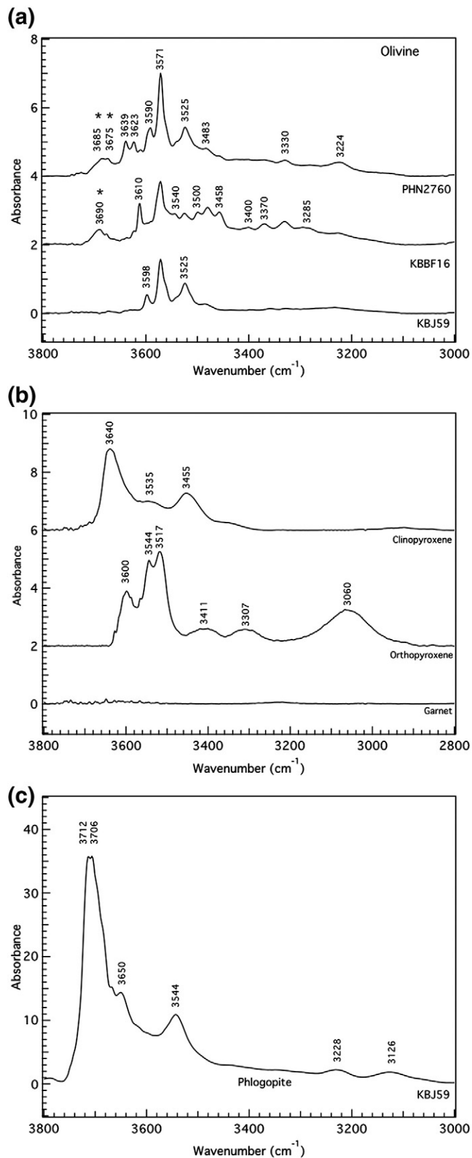
Fig. 8. Representative unpolarized infrared spectra of minerals in xenoliths from Kimberley and Jagersfontein. (a) Olivine. (b) Clinopyroxene, orthopyroxene, and garnet. (c) Phlogopite. All spectra are normalized to a sample thickness of 1 cm. Stars indicate peaks attributed to serpentine.
