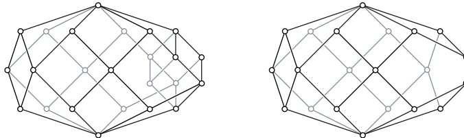
FIGURE 9.1. The bipartition-Cambrian lattices \mathcal{S}(3, 0) and \mathcal{S}(3, 1)
