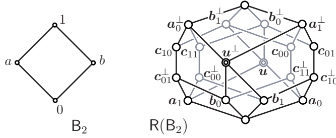
FIGURE 4.1. The lattice R(\mathbb{B}_2)
