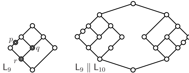
FIGURE 7.1. Bounded lattices with non-transitive join-dependency relation
