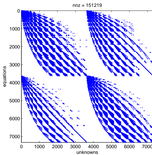
Figure 2: Distribution of the nonzero coefficients of P^0 .
