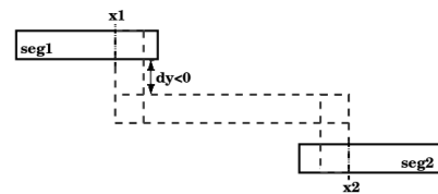
Fig. 10. Z-Shape routing, dy specified.
