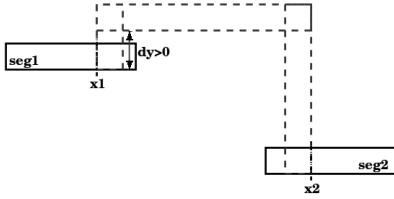
Fig. 12. U-Shape routing, dy > 0 specified.
