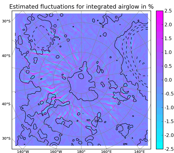
Figure 2: Airglow and gravity waves. Estimated fluctuations of integrated airglow intensity in %, derived from predictions with mesoscale model by [6] for southern polar regions around spring equinox. See [1] for further details.
