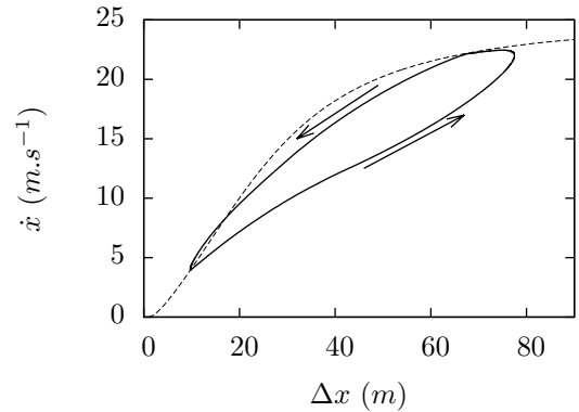
Fig. 5. Reaction of an IDM vehicle to a constraint varying between 4 \text{ m.s}^{-1} and 22 \text{ m.s}^{-1}
